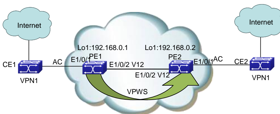
Fig 4-8 VPWS group network diagram
