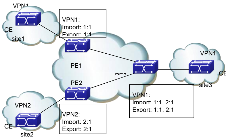
Fig 2-6 Extranet Networking Resolution
