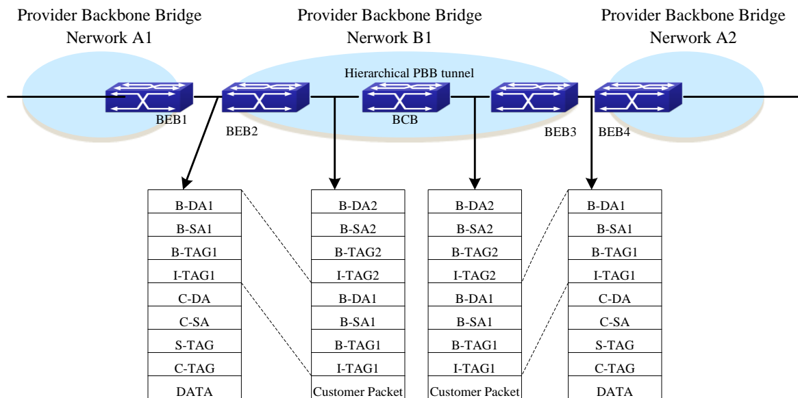
Fig 0-2 Basic Model of H-PBBN
