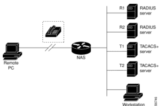
Figure 1-1 Typical AAA Network Configuration
