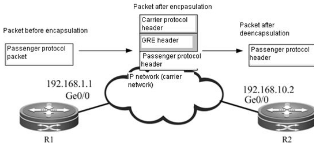
Figure 11 GRE tunnel
