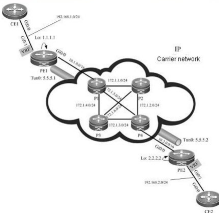
Figure 37 Network topology
