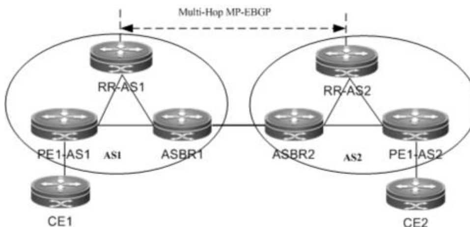
Figure 6 Setting up a multi-hop MP-EBG session between RRs in OptionC mode
