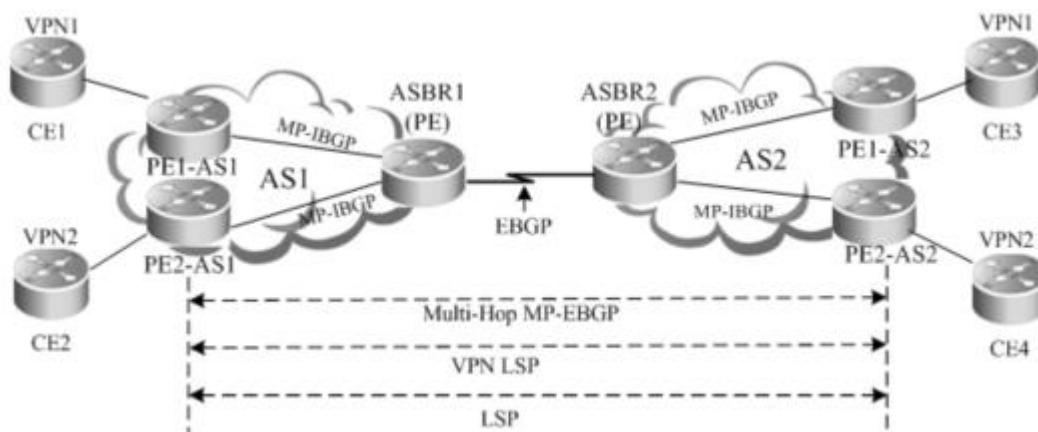
Figure 5 Multi-hope MP-EBGP
