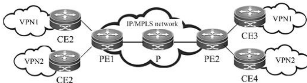
Figure 1 Basic components of a VPN
