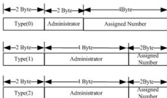
Figure 2 RD structure.
