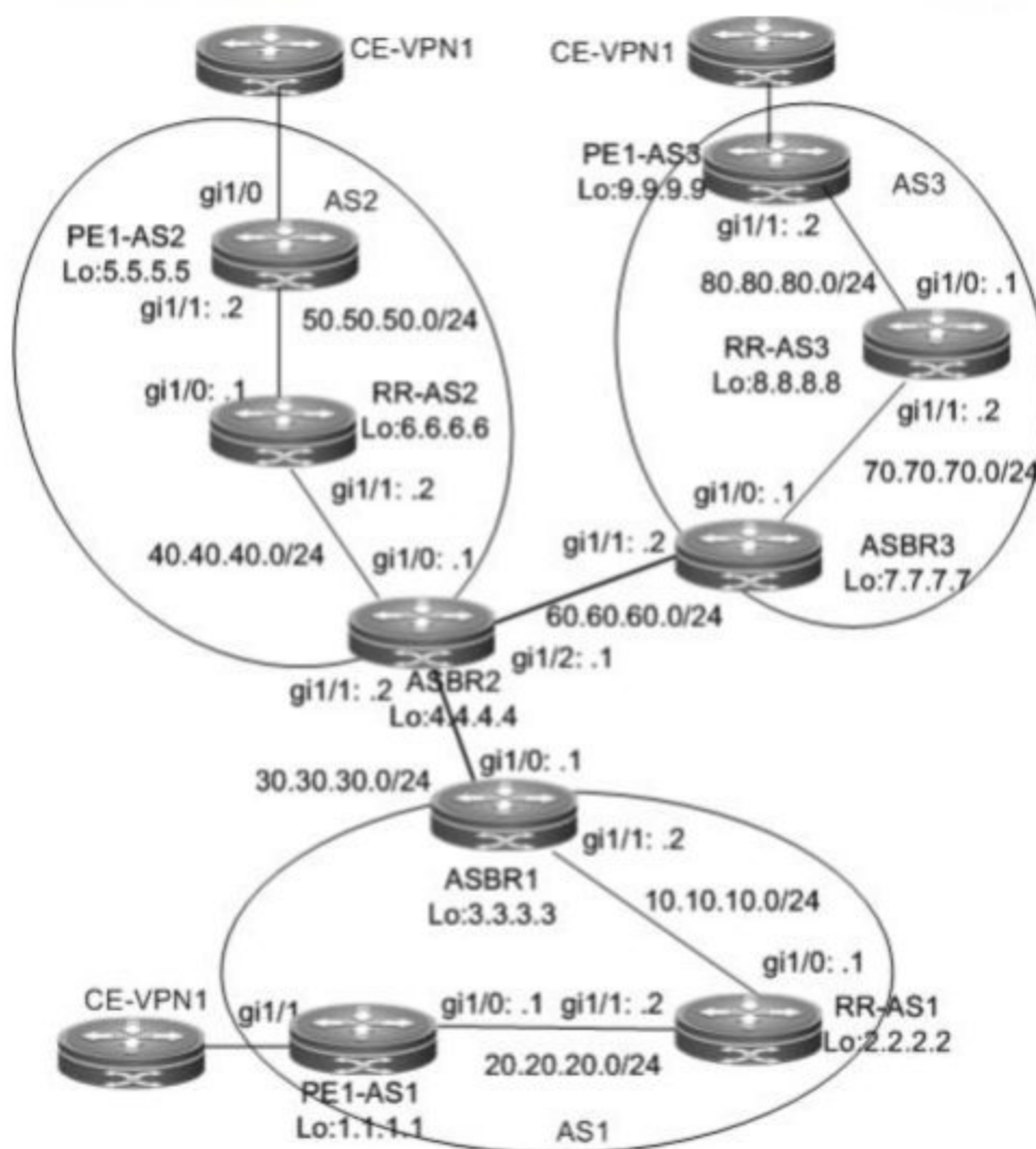
Figure 33 Setting up multi-hop MP-EBGP sessions between RR in the OptionC scheme
