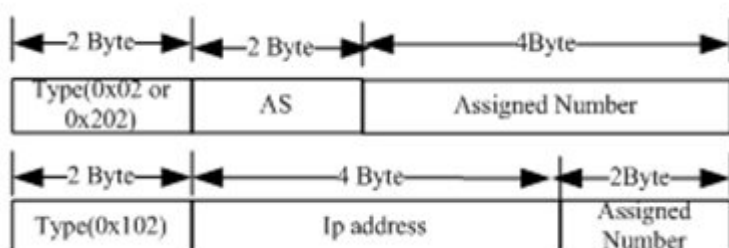
Figure 3 RT structure
