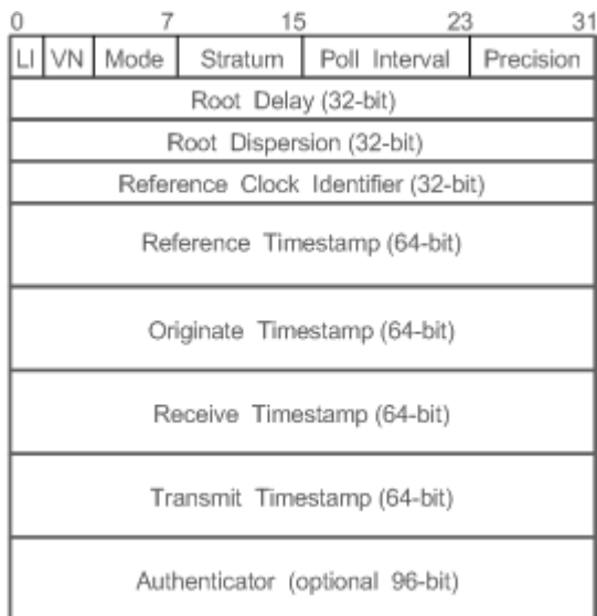
Figure 3-3 Format of an NTP Time Synchronization Packet
