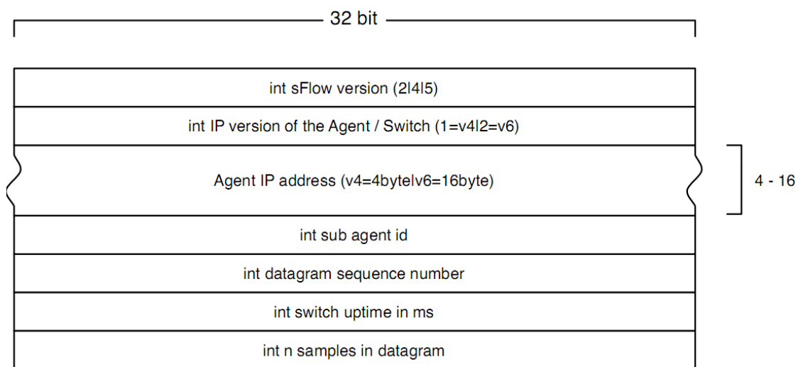
Figure 6-3 sFlow Header
