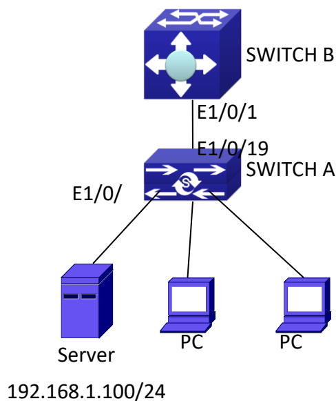
Fig 2-1 ARP scanning prevention typical configuration example
