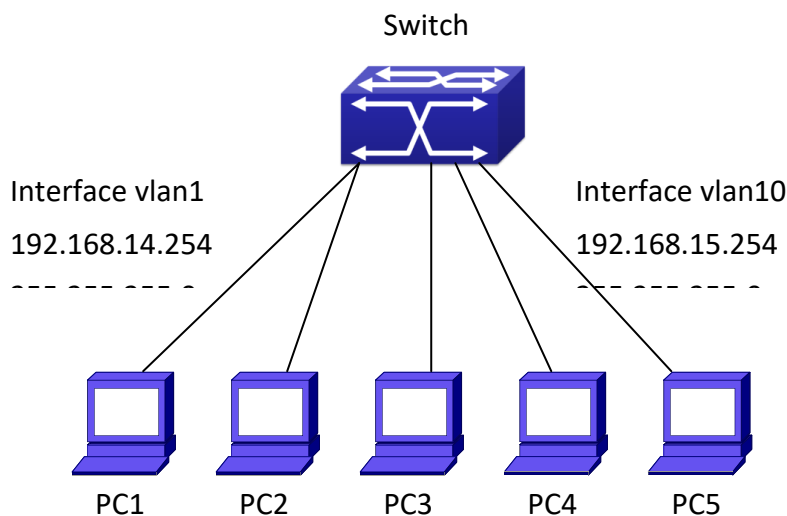
Fig 6-1 Gratuitous ARP Configuration Example
