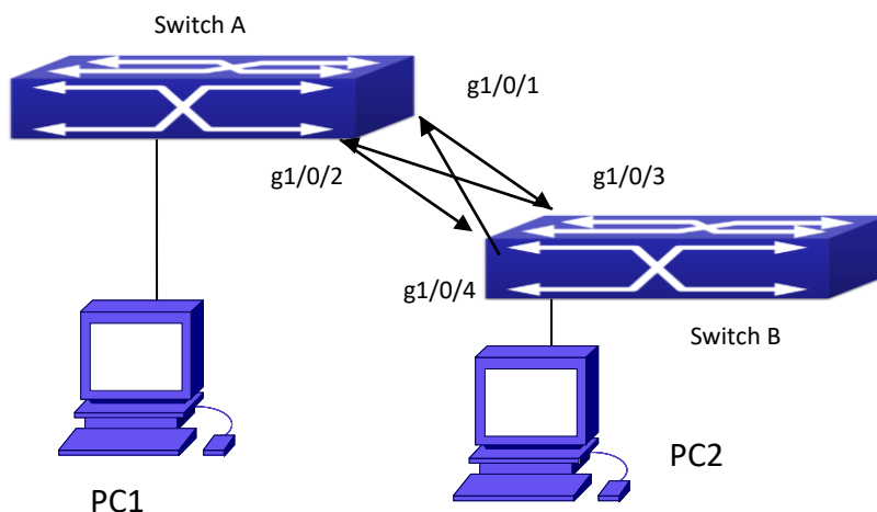
Fig 4-3 Fiber Cross Connection
