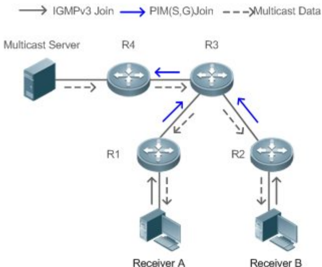
Figure 6-4 SSM Model
