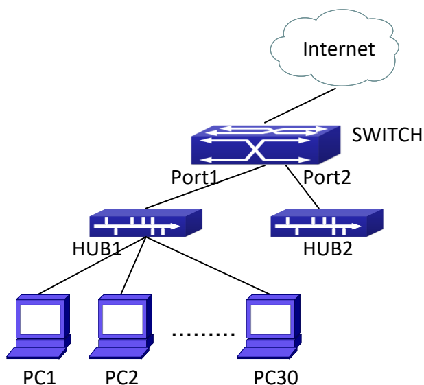
Fig 4-1 a typical configuration example of AM function
