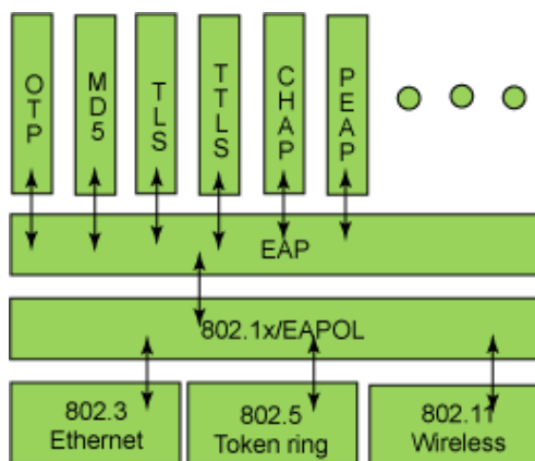
Fig 2-8 the Protocol Stack of EAP Authentication Method
