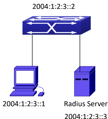
Fig 2-17 IPv6 Radius
